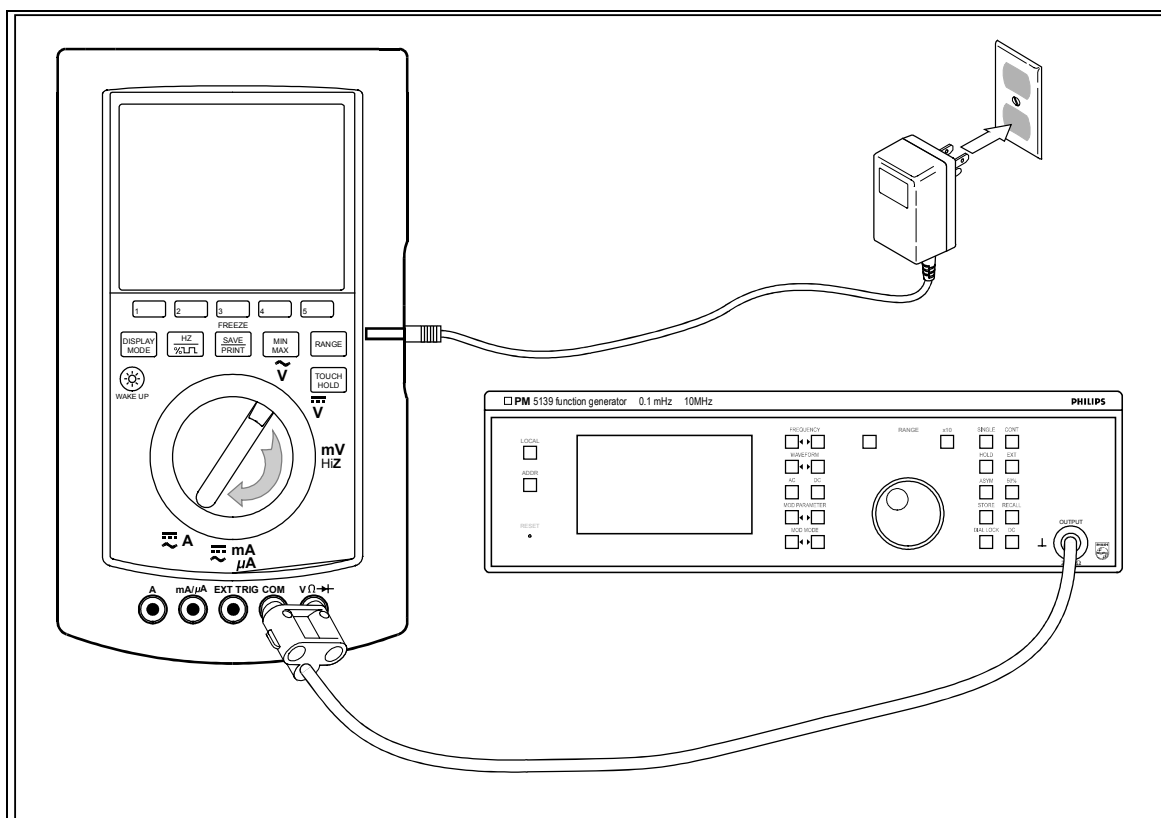
Figure 4-6. Configuration 10 (PM5139)
