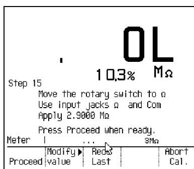
Figure 4-14. Ohms Calibration
