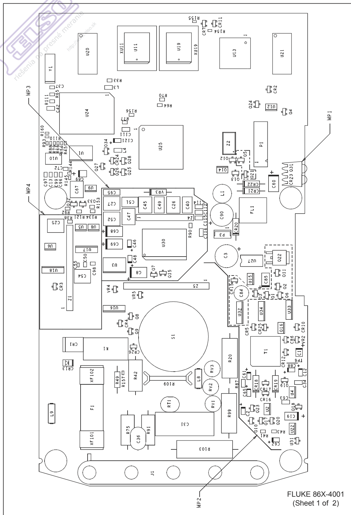
Figure 5-2. A1 Main PCA
