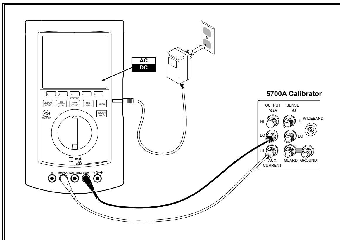
Figure 4-8. Configuration 3 (mAuA, DC and AC)
