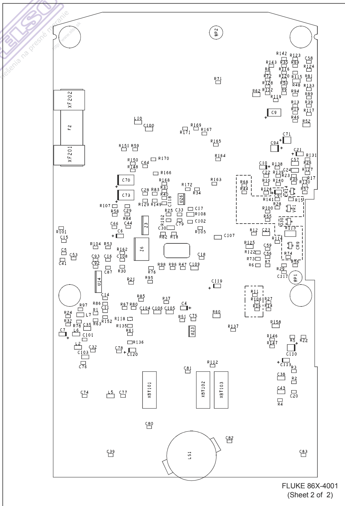
Figure 5-2. A1 Main PCA (cont)
