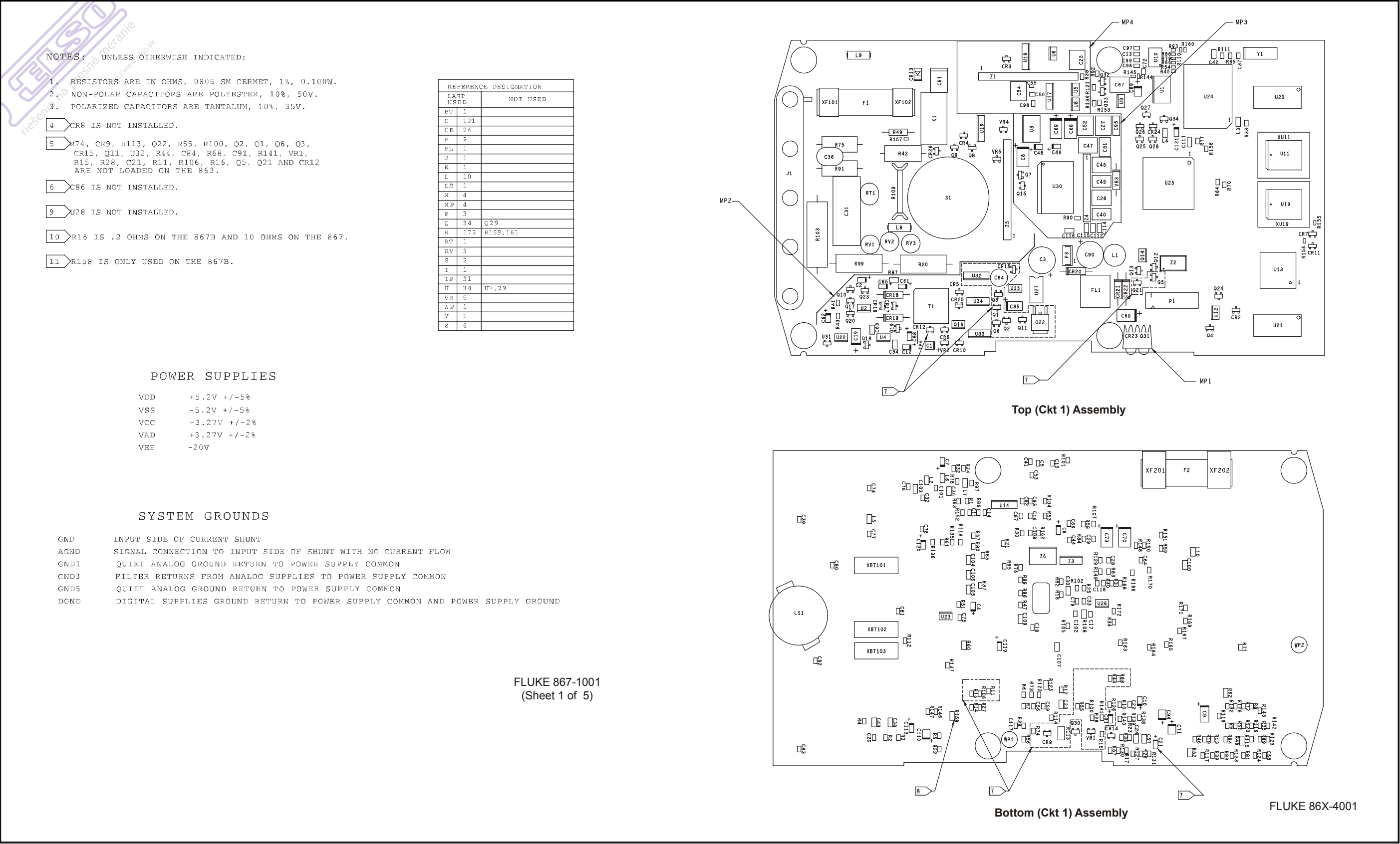
Figure 6-1. A1 Main PCA
