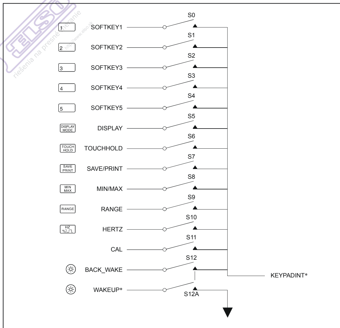
Figure 2-3. Keypad Connections
