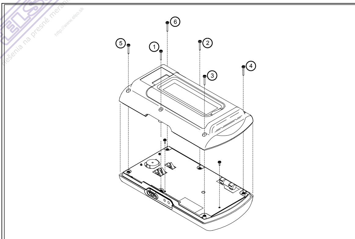
Figure 3-2. Reassembly
