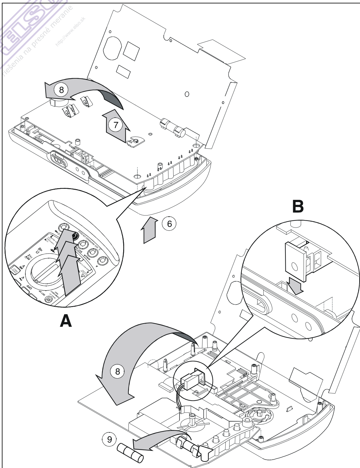
Figure 3-1. Disassembly (cont)
