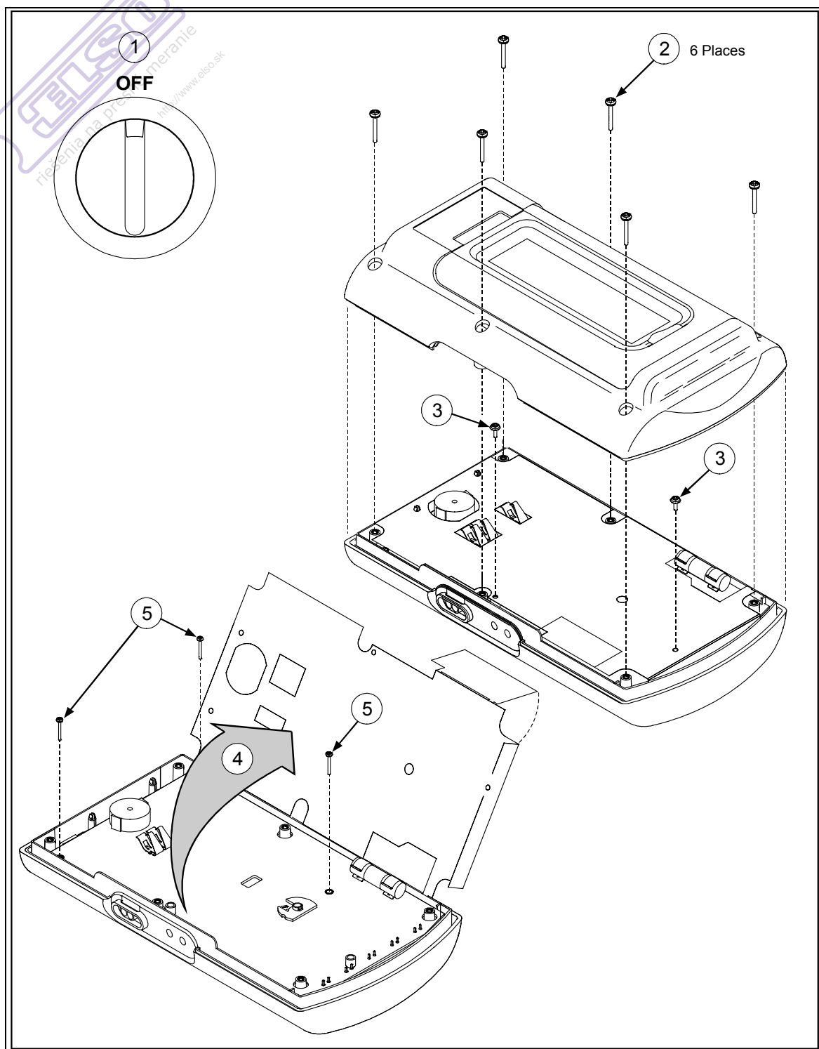
Figure 3-1. Disassembly
