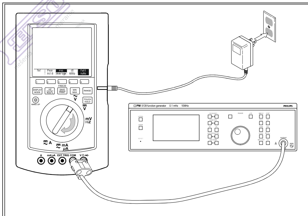
Figure 4-5. Configuration 7 (PM5139)
