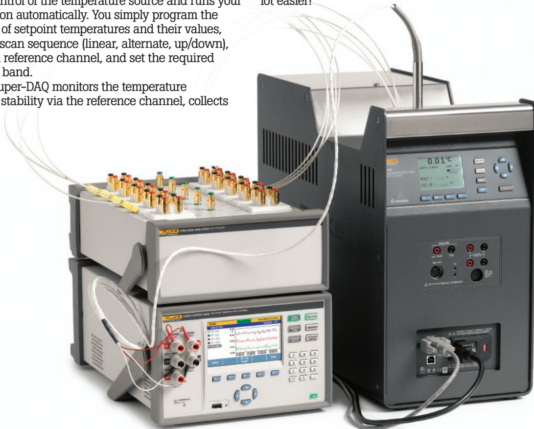
1586A configured with a DAQ-STAG and 9190A Ultra-Cool Field Metrology Well for automated sensor calibration.
