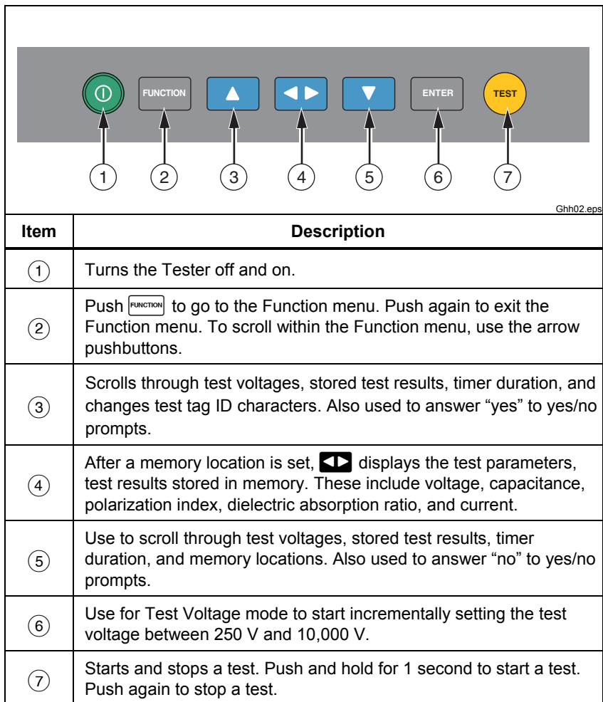
Figure 3. Pushbuttons
