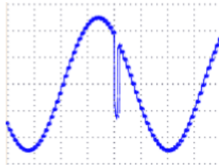
Waveform replayed at 950kHz repetition rate on 100MS/s DDS generator (output filter off). Note 10ns jitter visible on glitch.
