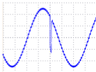
Waveform replayed at 950kHz repetition rate on 100MS/s variable clock generator (output filter off). For more information go to: www.tti-test.com/go/arb
