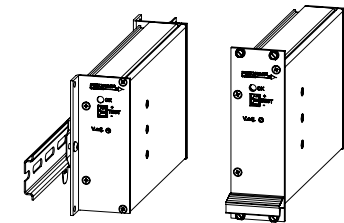
DIN-rail mounted Model with N + TS35 clips 19" subrack mounting Model with L-panel (opt.)
