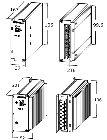
DIN or wall mounting Model with N (standard)
