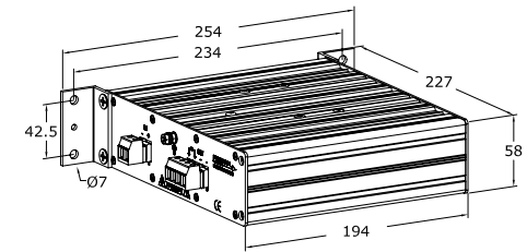
PM250/500 wallmounted. Brackets PL58-1 (standard)
