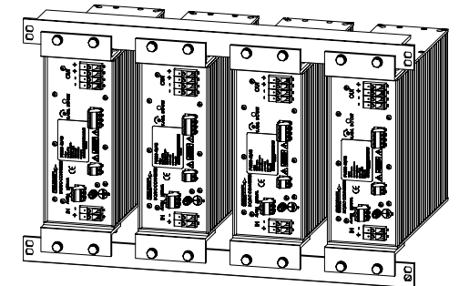
PU300/500 19" rack.
