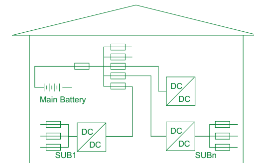
Sub-voltage supply with DC/DC converters
