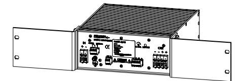
PU300/500 wallmounted. Brackets PL86-1 (standard)
