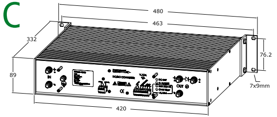
PU600/1000 Wallmounted. Brackets L89-1 (standard)
