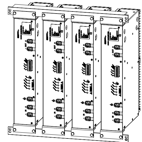
PC1000/2000 19" rack.
